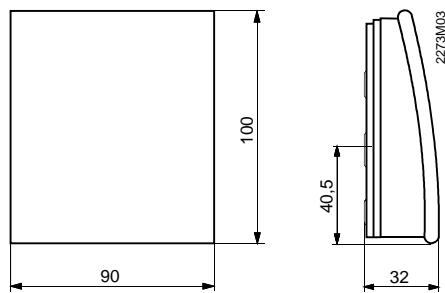
QAW44 remote temperature sensor
